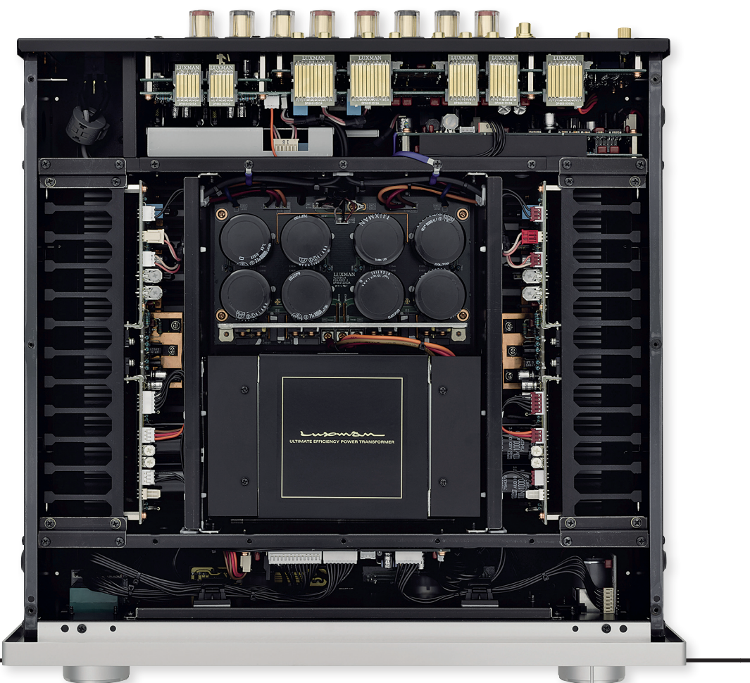
RIGHT: Massive 600VA frame transformer feeds mono power supplies and L/R audio stages, the preamp featuring an 88-step LECUA volume control feeding a three-stage parallel-output power amp mounted on huge, finned heatsinks
